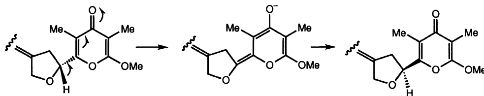
morpholine N -oxide (NMO) effected oxidation of 19 to aureonone 4 in moderate yield. Good accordance of synthetic 4 with an authentic sample was observed over the full range of the spectroscopic data and optical rotations { 4 : synthetic sample: [\alpha]_{\text{D}} -64.0^{\circ} ( \text{CHCl}_3 ), authentic sample: [\alpha]_{\text{D}} -56.9^{\circ} ( \text{CHCl}_3 )}. Based on this evidence, the absolute configuration of 4 , as well as that of 1 could be determined to be as depicted in Fig. 1.
