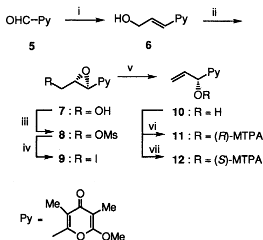
Scheme 1. reagents: i. a) \text{Ph}_3\text{P=CHCHO} ; b) \text{NaBH}_3\text{CN} (76%). ii. TBHP, \text{Ti}(\text{OPr}^i)_4 , L-DET (88%). iii. \text{MsCl} , pyr. (100%). iv. \text{NaI} (67%). v. \text{Zn} (88%). vi. ( S )-MTPACl, DMAP (100%). vii. ( R )-MTPACl, DMAP (95%).
